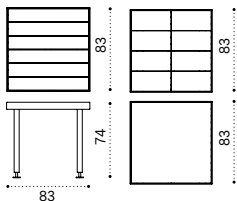
Dining table 83x83 h74 cm
